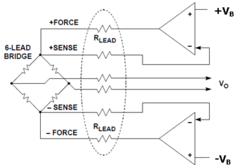
Figure 2: Balanced Bipolar 4-wire Kelvin Voltage Excitation
