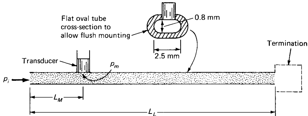
Figure 5-8: Diagram of a SIT Dynamic Pressure Measuring System
