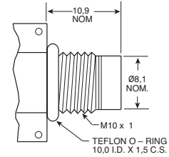
CTL-375M M10X1
