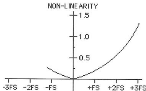
Figure 3-3: Independent Linearity Curve
